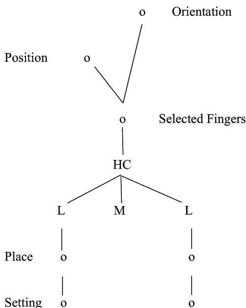
Fig. 15 Hierarchies of feature classes for Hand Configuration and Location (following Sandler 1989)
